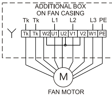
Fig. 2. Example electric connection diagram of WDV roof fans with three-phase motors (only star connection).
