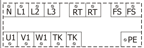
RTRD controller
