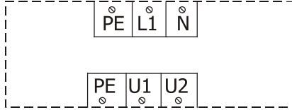
ARW controller
