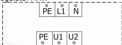
Rys. 53. Regulator ARW
